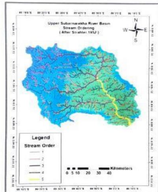
Figure 24: Stream ordering of the study area
